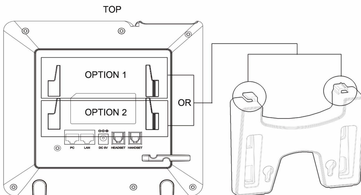
Figure 2: GXP16xx Stand Installation
