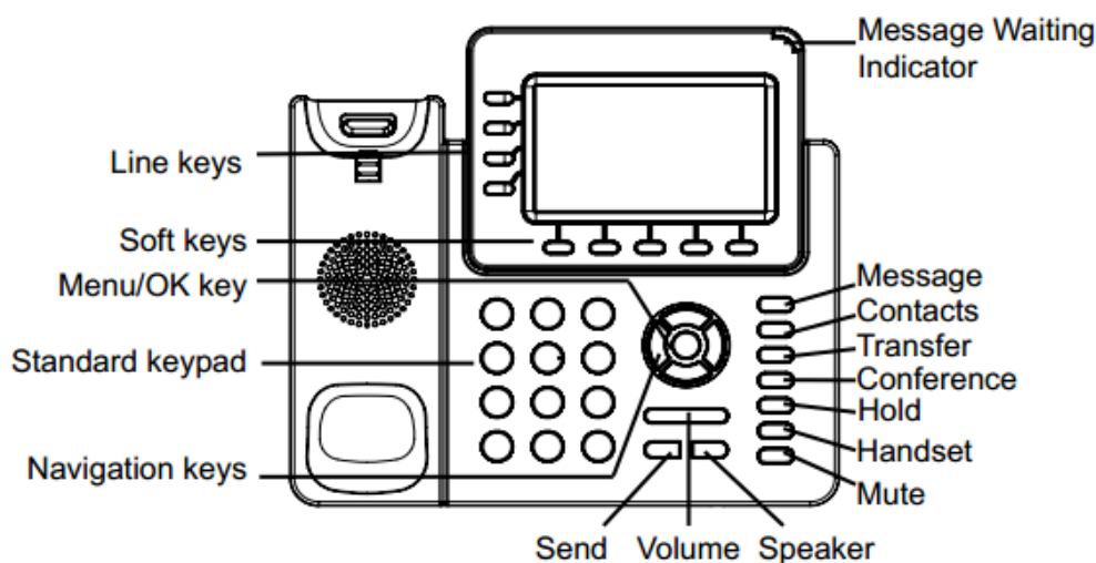
Figure 6: GXP2140 Keyboard
